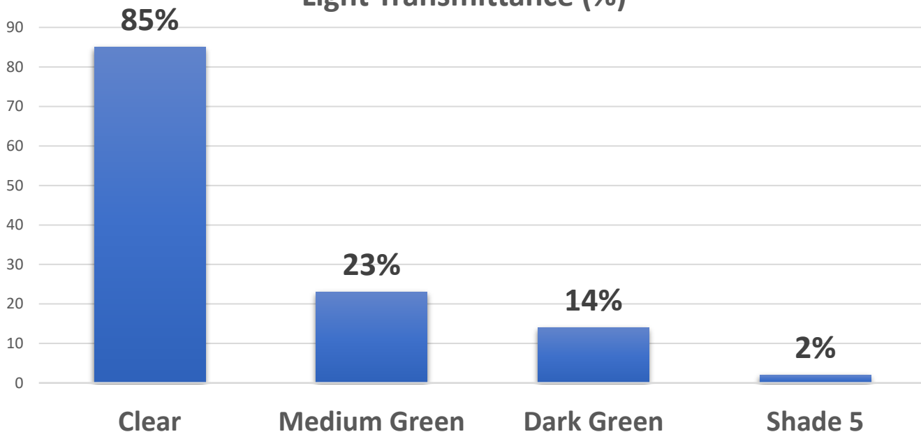
Light Transmittance (%)
